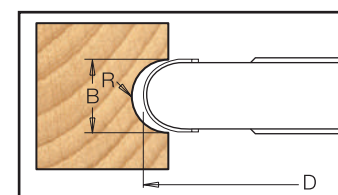
Option with Bearing
