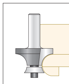
C.Molded Bearing #191 998 0S 18.5x6.3xR25.4
